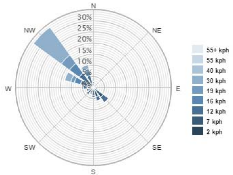
Windrose Speed Jun-Aug
