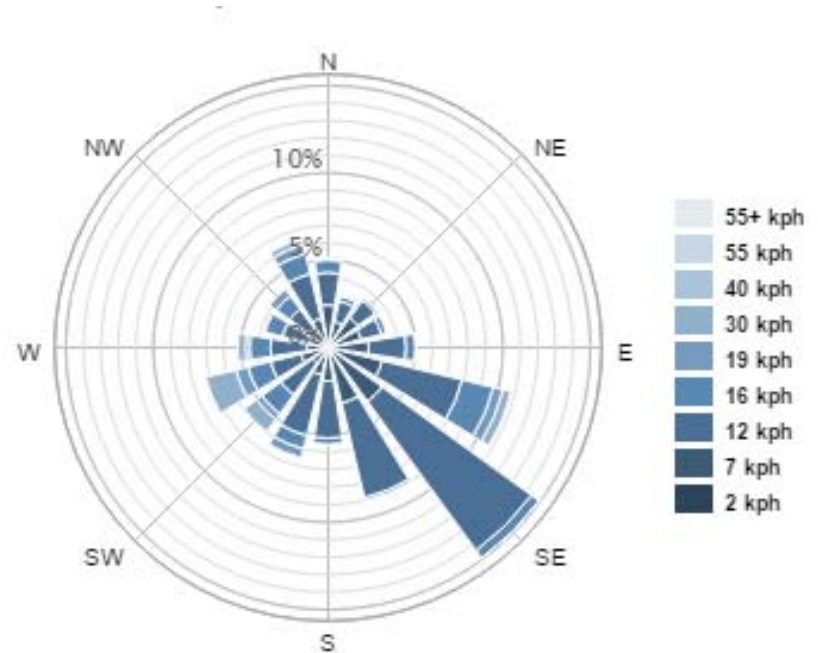
Windrose Speed Dec-Feb
