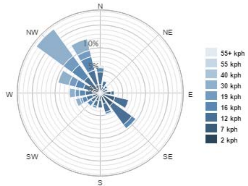
Windrose Speed Mar-May
