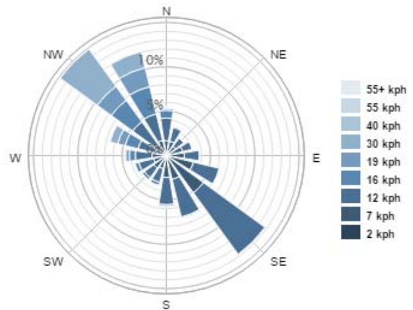
Windrose Speed Sep-Nov
